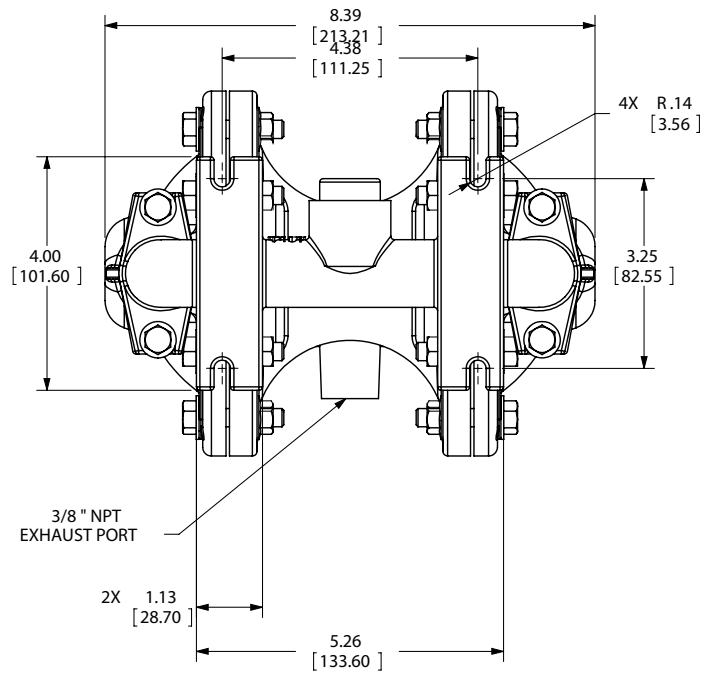
BOTTOM VIEW
