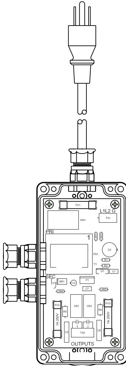
WIRING ILLUSTRATION Figure D
