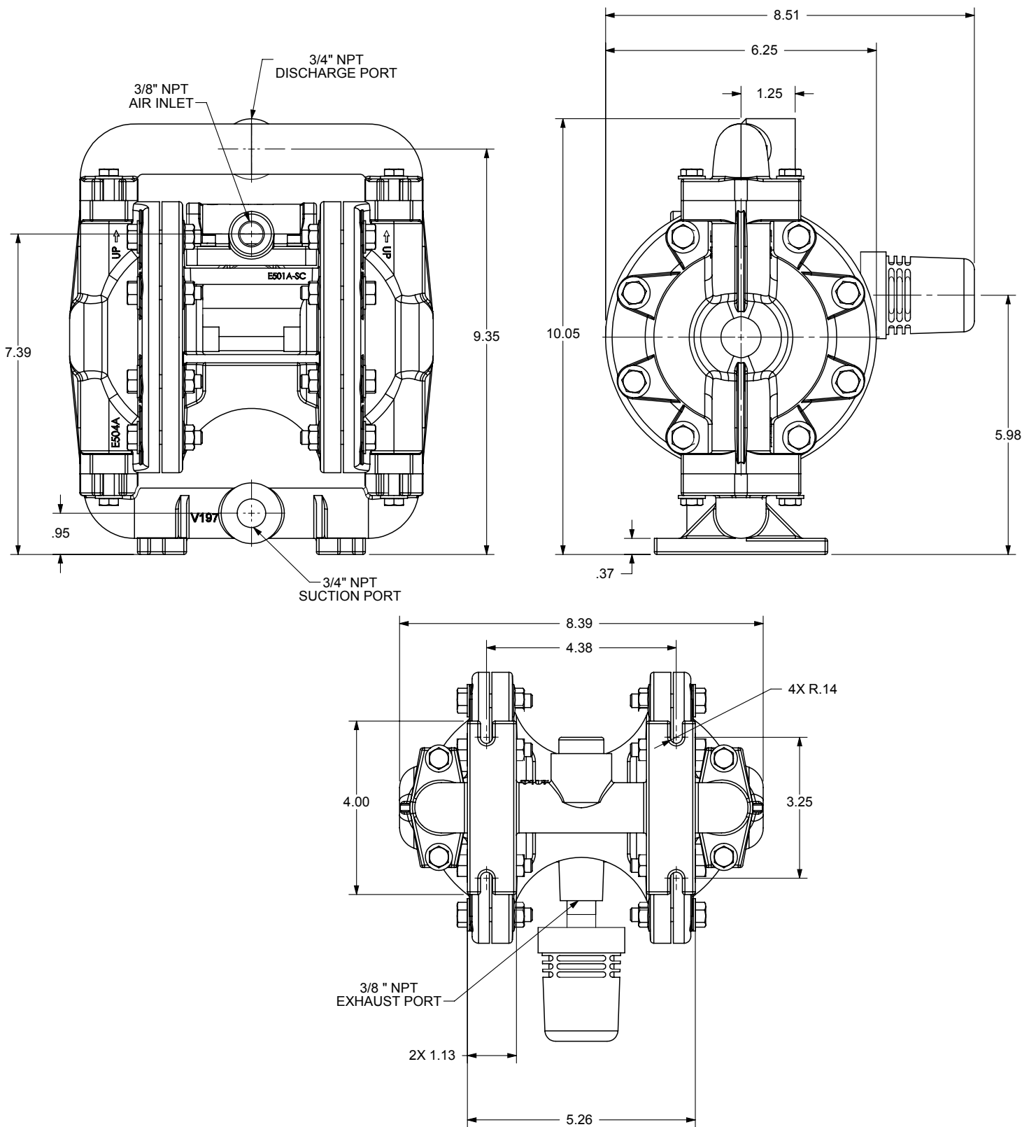
BOTTOM VIEW
